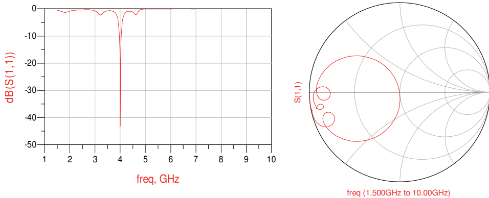
Fig. 13. Performance ( S_{11} and the smith chart) using \pi -network at 4 GHz.
