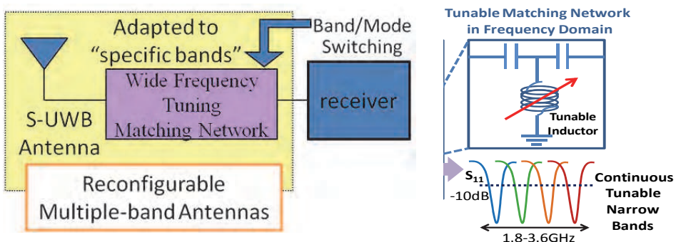
Fig. 1. The architecture of the reconfigurable multiband antennas.
