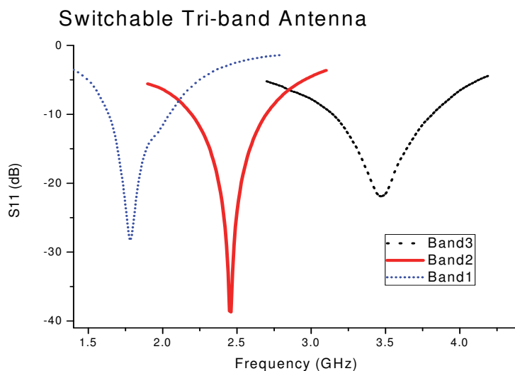
Fig. 14. S_{11} of the measured tri-band antenna.
