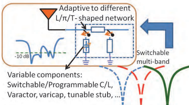
Fig. 2. System diagram of the band-switchable antennas.
