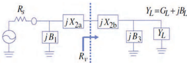
Fig. 8. The mediate step reconfigurable multiband analog antennas.
