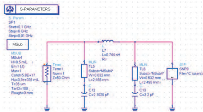
Fig. 6. ADS simulation combined tunable matching network and an S-UWB antenna (SIP).
