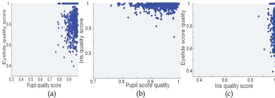
Fig. 9. Illustration of the correlations between different quality scores: the measures are not grouped on the diagonal, therefore they are uncorrelated
