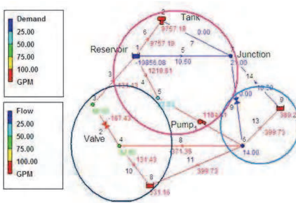
Fig. 11. Grouped nodes in the topology.
