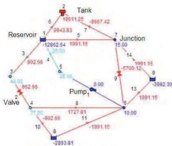
Fig. 16. Topology of simulation for all reservoirs are serving.
