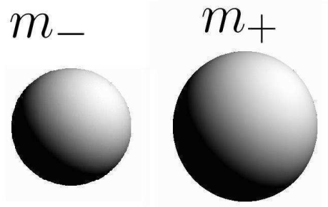
Fig. 3. Light and heavy fermion species of Lagrangian 25. Adapted from Ref. (Hernández Ortíz, 2011).
