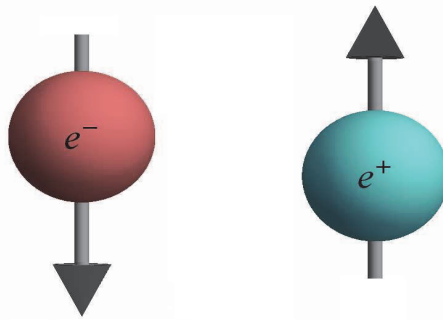
Fig. 2. The particle spectrum of solutions to the Dirac equation in Eq. (11). Adapted from Ref. (Hernández Ortíz, 2011).
