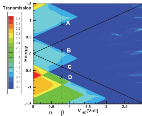
Fig. 7. Contour plot of transmission with respect to the energy and V_{sd} for the system size (N, M) = (4, 6) and the applied gate voltage V_g = 0.5 V. Dashed Oblique lines shows the current integration window. Points marked by A, B, C, D correspond to the horizontal lines with the same name in Fig.(2). Lines of \alpha, \beta are the trace of points with similar names in Fig.(6). Fermi energy was fixed at zero E_F = 0 .
