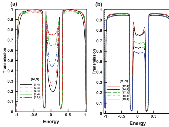
Fig. 5. Transmission through graphene ribbon with 4 zigzag chains in width for different ribbon lengths: a) M \leq 12 b) M \geq 12 . Applied bias is considered to be 0.5V. Edge impurity changes onsite energy of the edge atoms as \epsilon_\alpha = 0.1t .
