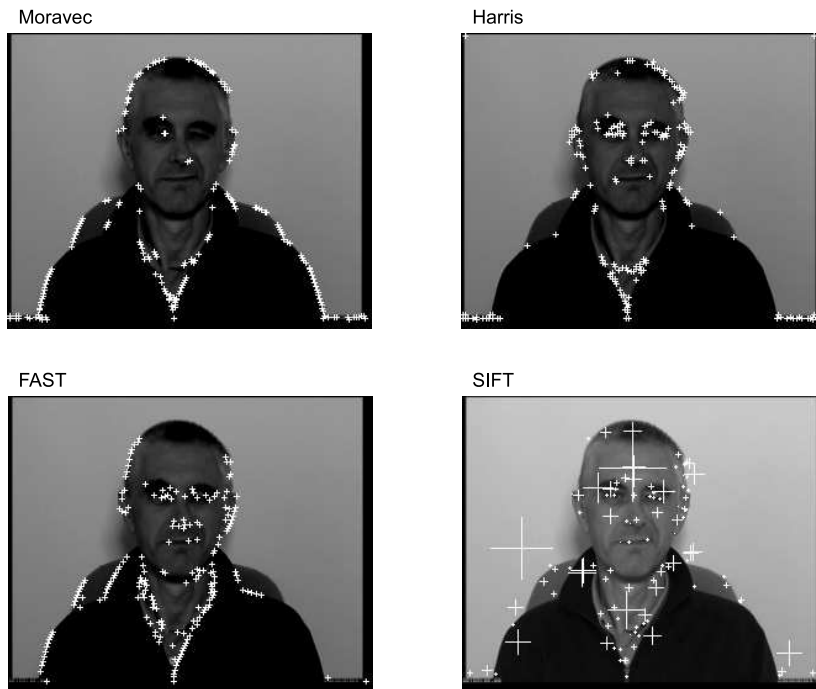
Fig. 4. Results of different corner detectors.
