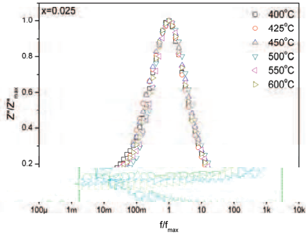
Fig. 6. Scaling behaviour of Z'' at various temperatures.
