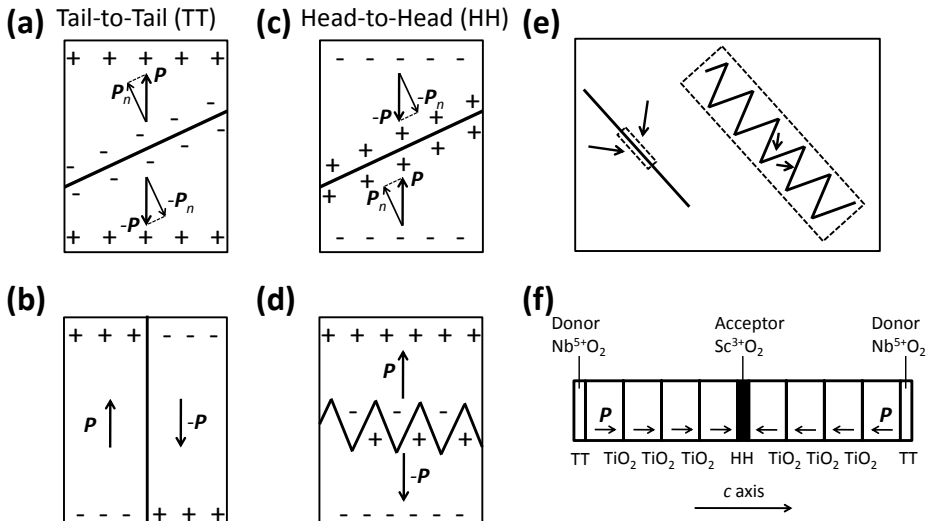
Fig. 3. (a) Tail-to-tail, (b) uncharged, (c) head-to-head and (d) charged zigzag 180° merohedral domain boundaries. The boundary (b) is also common among pseudo-merohedral domain boundaries. Figures (a) to (d) after ref. (Hahn & Klapper, 2003). Panel (e) shows the 90° pseudo-merohedral domain boundary which at first glance appears as a head-to-head domain boundary, but in a detailed study turned out to be a zigzag boundary where all boundaries are head-to-tail, shown in the right-hand corner. Figure after ref. (Lines & Glass, 1998; Yakunin et al, 1972). Panel (f) shows a ferroelectric superlattices used in a first-principles computational study in which head-to-head and tail-to-tail domain boundaries are stabilized by placing donor and acceptor layers to serve as charge compensation layers (Wu & Vanderbilt, 2006).
