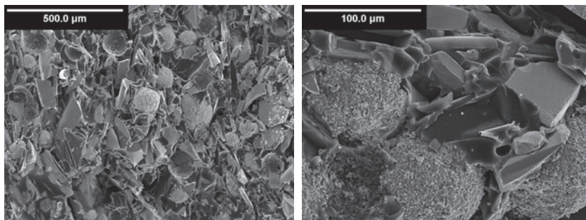
Fig. 9. SEM micrographs of hybrid magnetic composite materials
