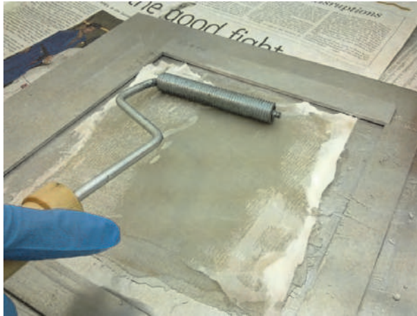
Fig. 4. Wet layup of silk fabric
