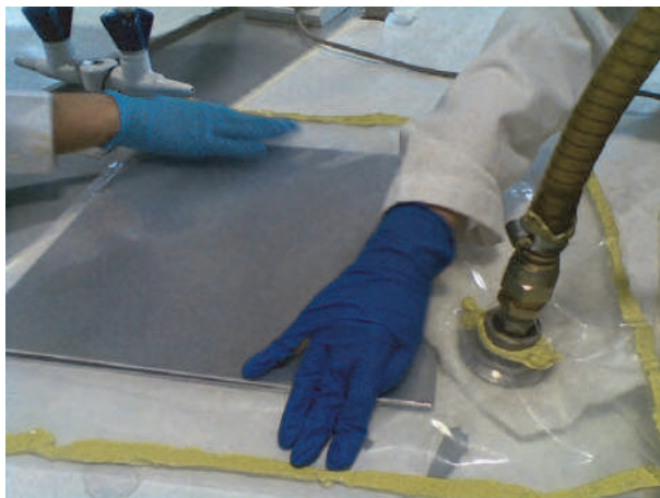
Fig. 5. Vacuum Bagging Setup
