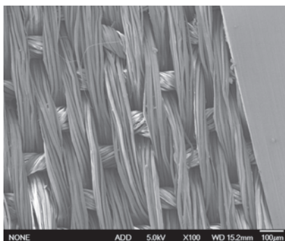
Fig. 2. SEM Analysis of Woven Silk Fabric.
