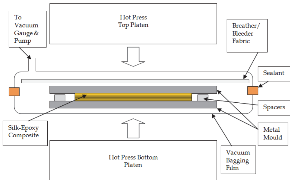
a) Detailed schematics of hot press setup
