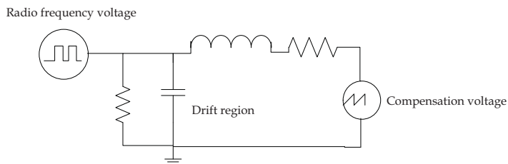
Fig. 14. Compensation voltage connection diagram
