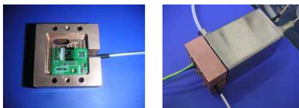
Fig. 21. Photos of the MEMS Faraday cup packaged
