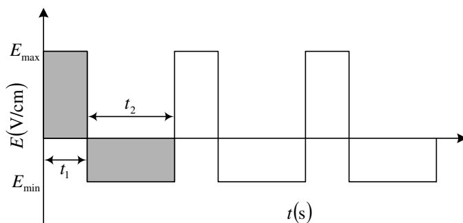
Fig. 7. Electric field of asymmetric waveform
