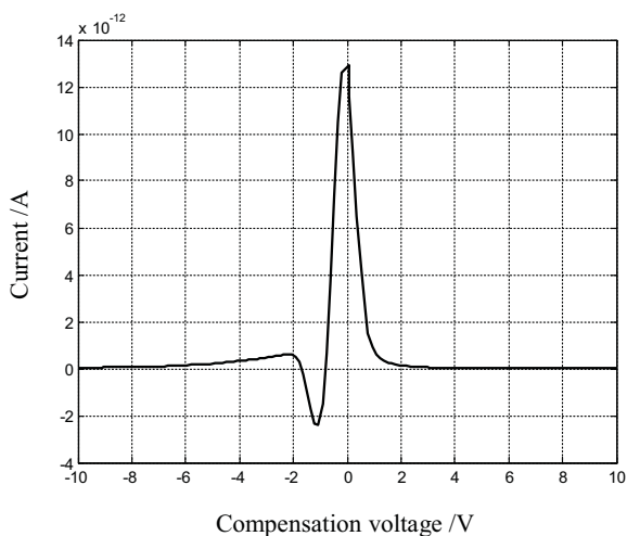
Fig. 35. FAIMS Spectrogram of 0.1ppm acetic acid
