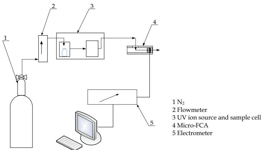
Fig. 22. Experimental apparatus of the MEMS Faraday cup
