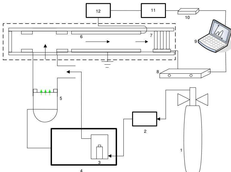
1 Nitrogen tank, 2 Flowmeter, 3 Sample cell, 4 Ion source power, 5 Ultraviolet lamp, 6 Drift region, 7 Column array micro Faraday cup, 8 Amperometer, 9 Computer, 10 Collection card, 11 Compensation voltage, 12 Square wave radio frequency voltage
