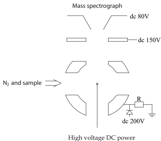
Fig. 10. Mass spectroscopic circuit diagram under the mode of positive ionisation
