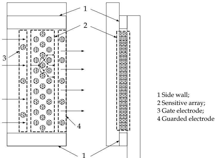
Fig. 16. Structure of the MEMS Faraday cup
