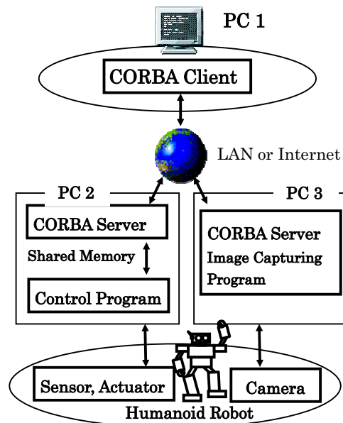
Figure 39. Teleoperation concept
