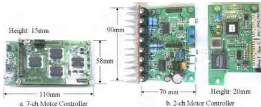
Figure 9. Servomotor Controllers
