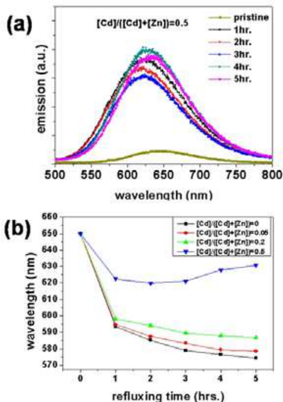
Fig. 3.13. Temporal change of (a) photoluminescence spectra and (b) emission wavelength of \text{Cu}_{1-x}\text{InS}_2 nanocrystals ( x=0.8 ) the surface modified with alloyed capping layers.
