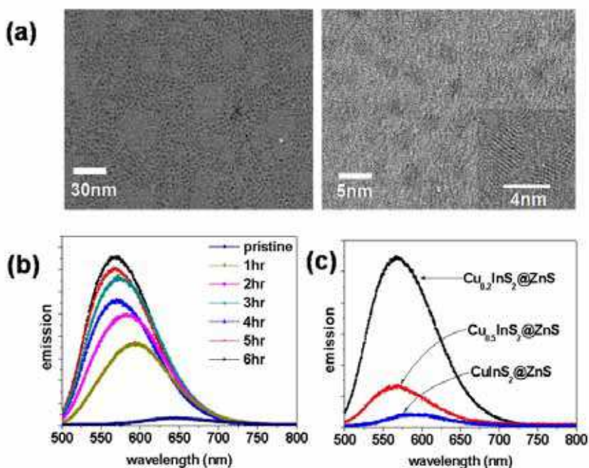
Fig. 3.10. (a) TEM images of \text{Cu}_{1-x}\text{InS}_2 nanocrystals ( x=0.8 ) treated with zinc acetate and palmitic acid for 5 hours at 230^\circ\text{C} . (b) Temporal evolution of PL of \text{Cu}_{1-x}\text{InS}_2 nanocrystals ( x=0.2 ) (c) PL of \text{Cu}_{1-x}\text{InS}_2 NCs with various starting composition ( x=0, 0.5, 0.8 ) after refluxing with zinc acetate and palmitic acid for 5 hours at 230^\circ\text{C} .
