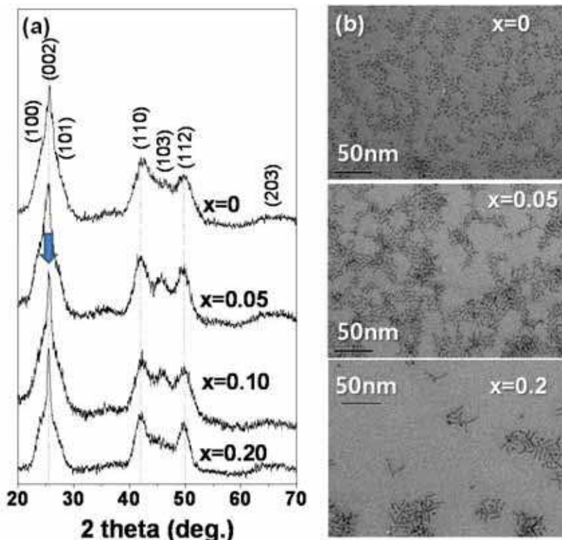
Fig. 2.1. (a) X-ray diffraction (XRD) patterns and TEM images of nanocrystals grown at 225°C with various initial molar abundance of Pb, x = \text{Pb}/(\text{Cd} + \text{Pb}) . Peak indices in the XRD pattern were assigned according to wurzite CdSe.
