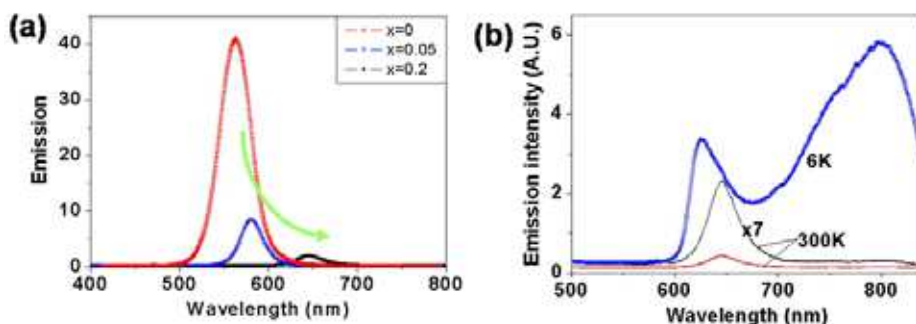
Fig. 2.4. (a) Room temperature photoluminescence of \text{Cd}_{1-x}\text{Pb}_x\text{Se} with various Pb-content( x ) and (b) temperature dependence of photoluminescence spectra for \text{Cd}_{1-x}\text{Pb}_x\text{Se} ( x=0.2 ) nanocrystals grown at 225^\circ\text{C} .
