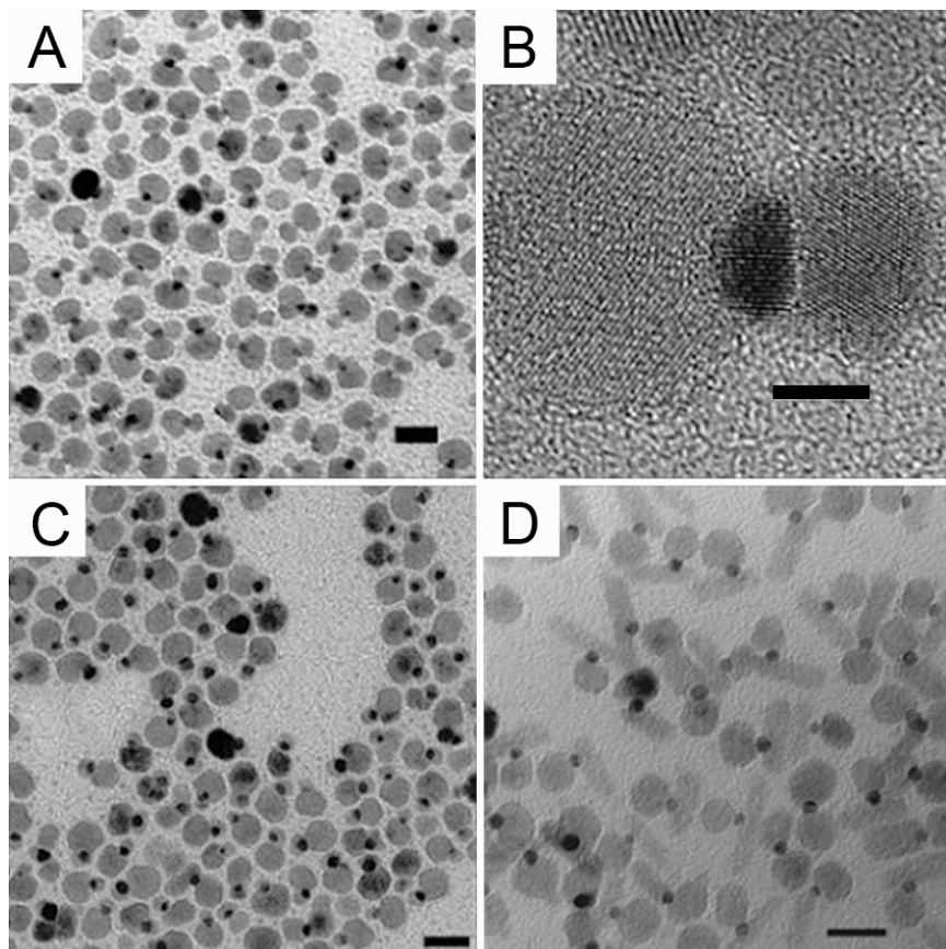
Fig. 10. (A) TEM and (B) High-resolution TEM images of \text{Fe}_3\text{O}_4 -Au-PbSe ternary hybrid nanostructure. (C-D) TEM images of \text{Fe}_3\text{O}_4 -Au-PbS ternary hybrid nanostructure. The scale bars are 20 nm in (A), (C), and (D) and 4 nm in (B). Courtesy: Nano Lett., 2006, 6, 875-881.
