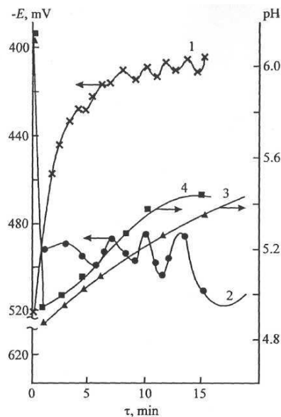
Fig. 6. Temperature dependencies of electrochemical potential (1, 2) and pH (3, 4) at 20 °C (1, 3) and 40 °C (2, 4); 0.01 wt.% \text{H}_2\text{O}_2 .
