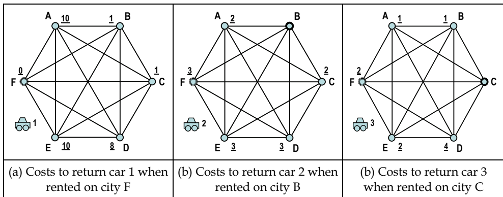
Fig. 2. Return costs
