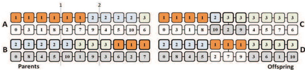
Fig. 5. Recombination operator
