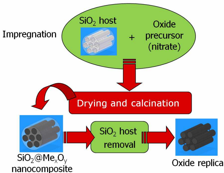
Fig. 9. Sketch of nanocasting pathway for the synthesis of \text{SiO}_2@Me_xO_y nanocomposites. Further selective etching of the \text{SiO}_2 matrix releases the Me_xO_y as a negative replica of the \text{SiO}_2 host.
