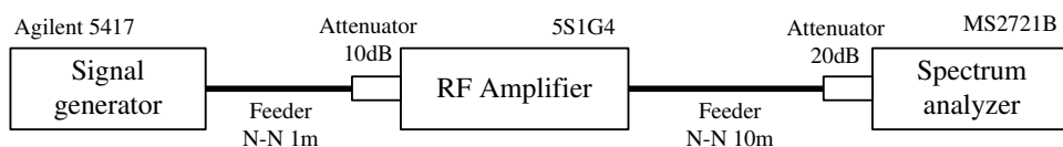
Fig. 3. Transmitting section calibration set schematic diagram
