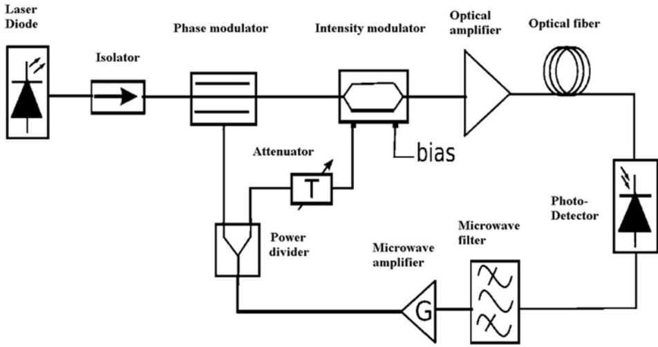
Fig. 5. Topology with compression of impulsion
