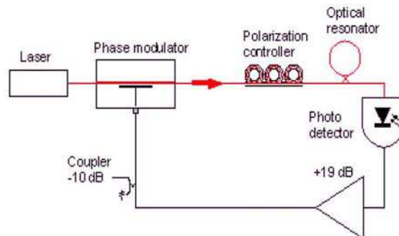
Fig. 6. Typical architecture of an optical resonator based OEO realized at FEMTO-ST institute
