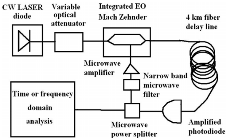
Fig. 1. Typical architecture of a fiber delay line OEO realized at FEMTO-ST institute
