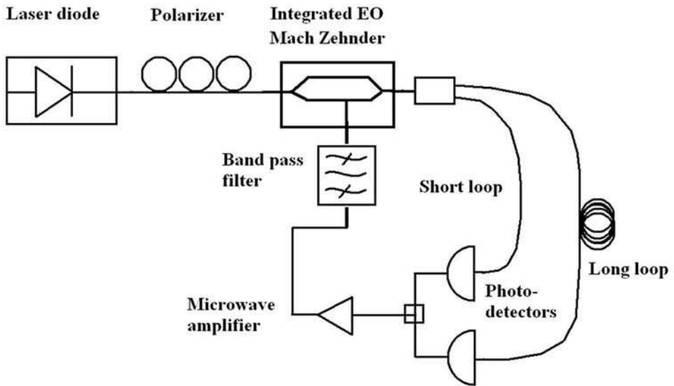
Fig. 3. Double loop topology of OEO
