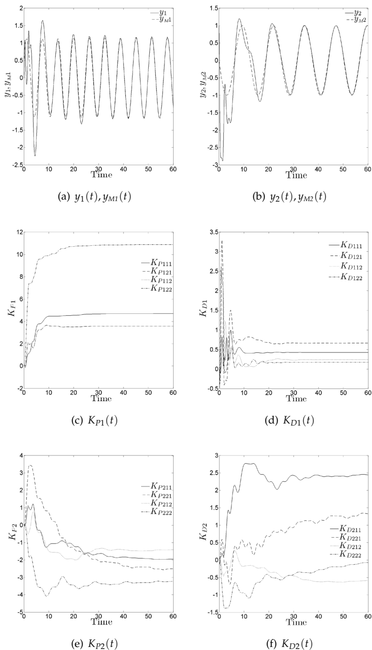
Fig. 3. Simulation Results of Example 2
