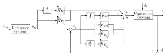
Fig. 1. Proposed Adaptive PID Controller
