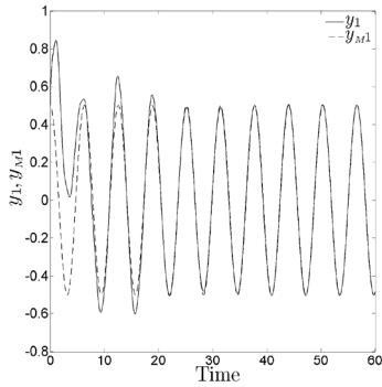
(a) y_1(t), y_{M1}(t)
