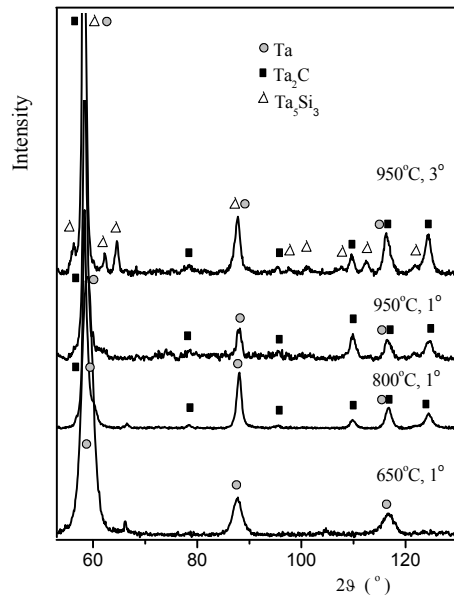
Fig. 14. Grazing angle XRD spectra with Cr k_\alpha radiation of Ta/SiC after annealing in vacuum. The thickness ratio of Ni:Ta is \sim 3:5 and the total film thickness is \sim 100 nm.
