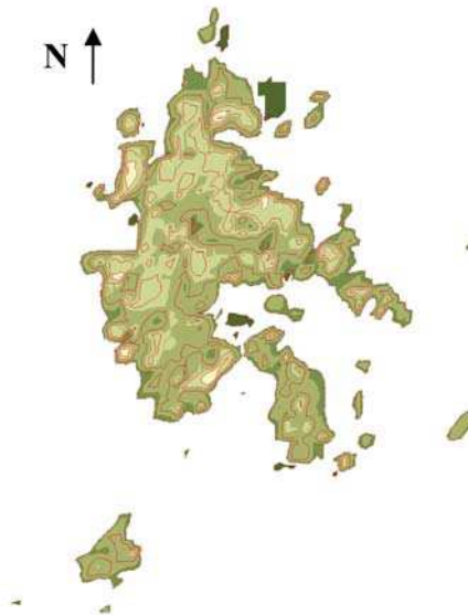
Fig. 4. Urban Potential for Great Mendoza (1990/92) in equipotential contour lines format.
