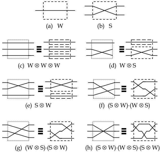
Fig. 13. Many-valued ( m -ary) reversible and conservative permutation-based circuits: (a) m -ary (1, 1) Wire (W), (b) m -ary (2, 2) Swap (S), and (c) - (h) all possible m -ary reversible and quantum (3, 3) Swap-based primitives. The symbol \otimes is the Kronecker (i.e., tensor) product.
