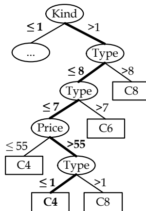
Fig. 10. Example of a classification decision tree
