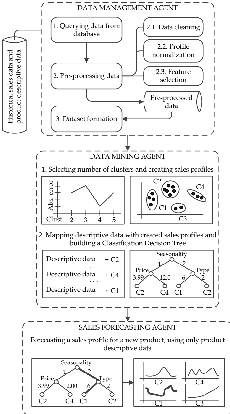
Fig. 8. Multi-Agent System for Sales Forecasting
