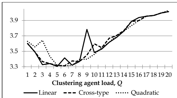
Fig. 5. Learning error (MAE) in periods for the system with SOM algorithm, using MEuclidean
