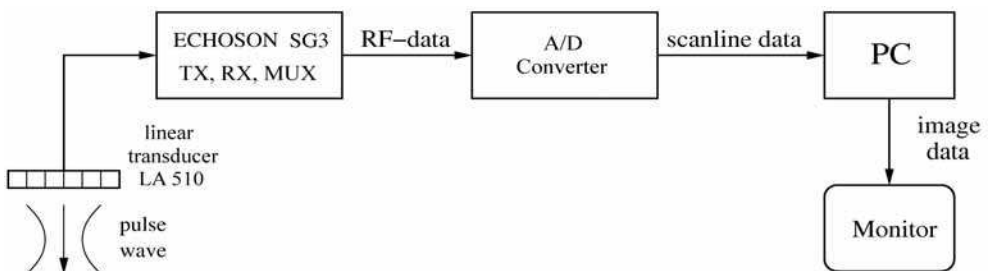
Fig. 11. Block diagram of the ultrasound imaging system
