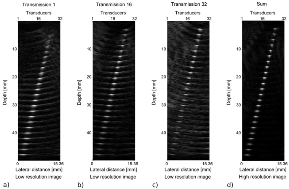
Fig. 13. Low resolution images combined to produce a high resolution image. One element transmit at the time, while all are used to receive. The images are then added into one high resolution image
