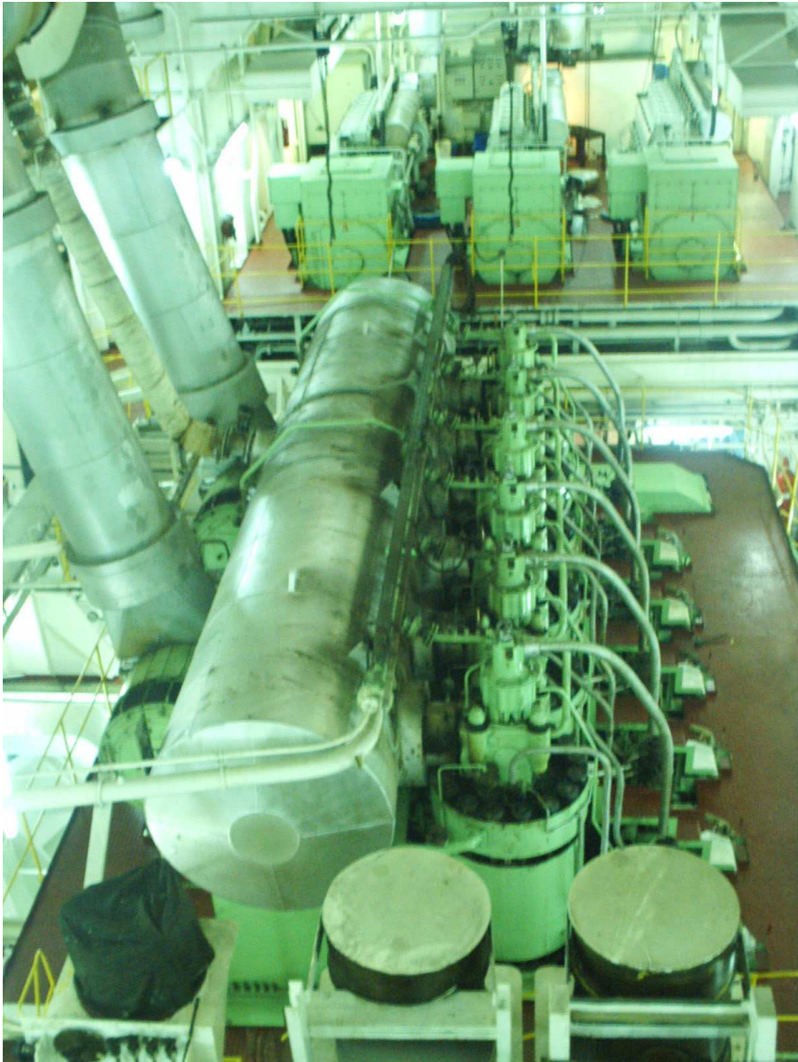
Fig. 3. Main engine
