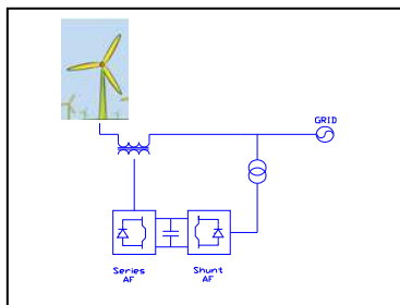
Fig. 6. Scheme of Unified Power-Quality Conditioner.
