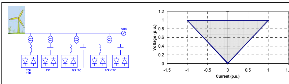
Fig. 3. Different topologies of SVC and V-I characteristic.
