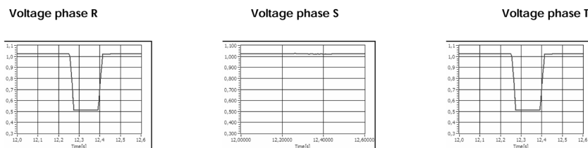
Fig. 16. Two-phase voltage dip: Depth 50%; Duration 150 ms.
