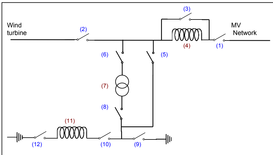
Fig. 14. Scheme of the voltage dip generator.
