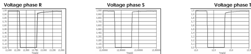
Fig. 15. Three-phase voltage dip: Depth 100%; Duration 510 ms.
