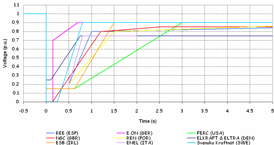
Fig. 1. Fault ride through requirements.
