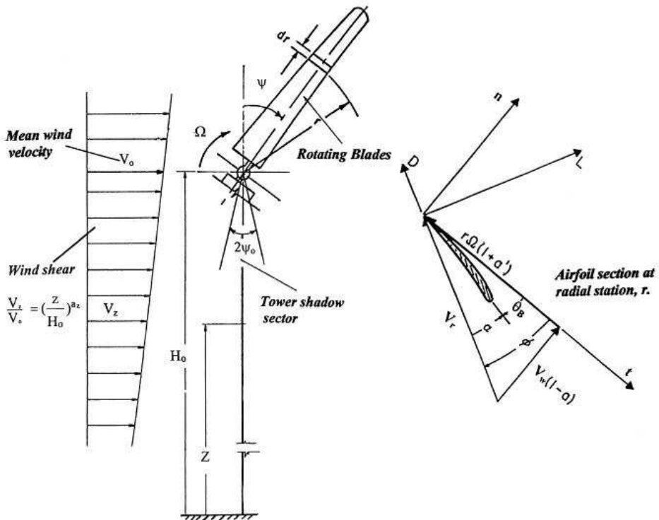
Fig. 3. Wind rotor geometry and velocity components
