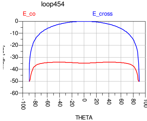
Fig. 23. Loop Antenna Radiation pattern on human body
