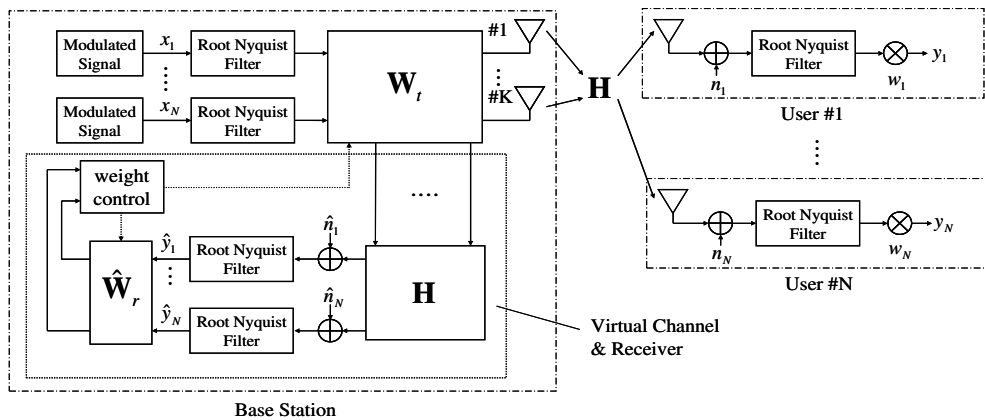
Fig. 12. System configurations
