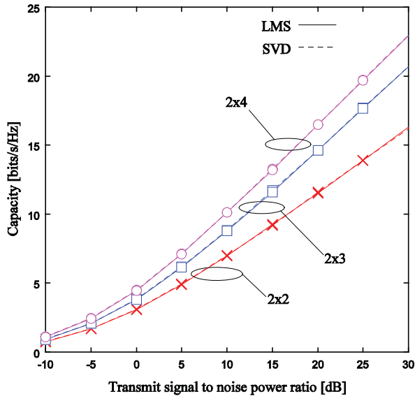
Fig. 10. Channel capacity performance (2xN r )
