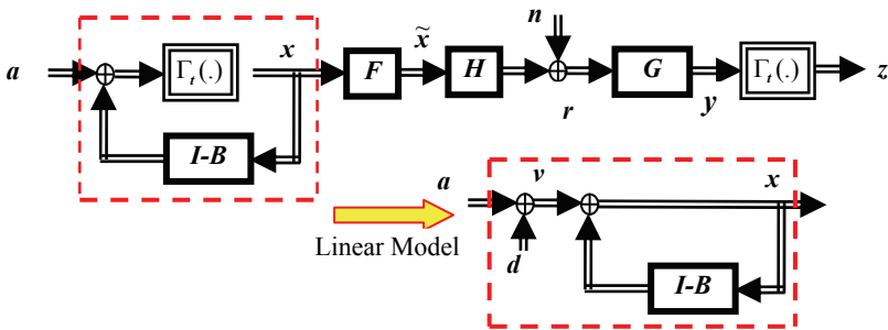
Fig. 1. THP model in a MIMO system
