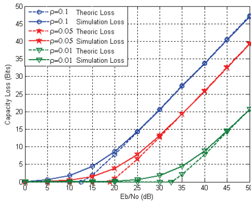
Fig. 9. Capacity loss for K=4 user
