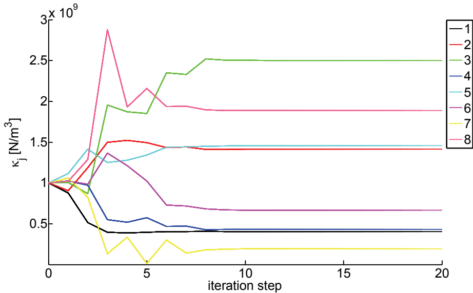
Fig. 6. Evolution of the stiffness parameters \kappa_j ( j=1,\dots,8 in the legend) during iterations by adopting the proposed updating procedure. Example with 12 measurement response dofs and without noise.
