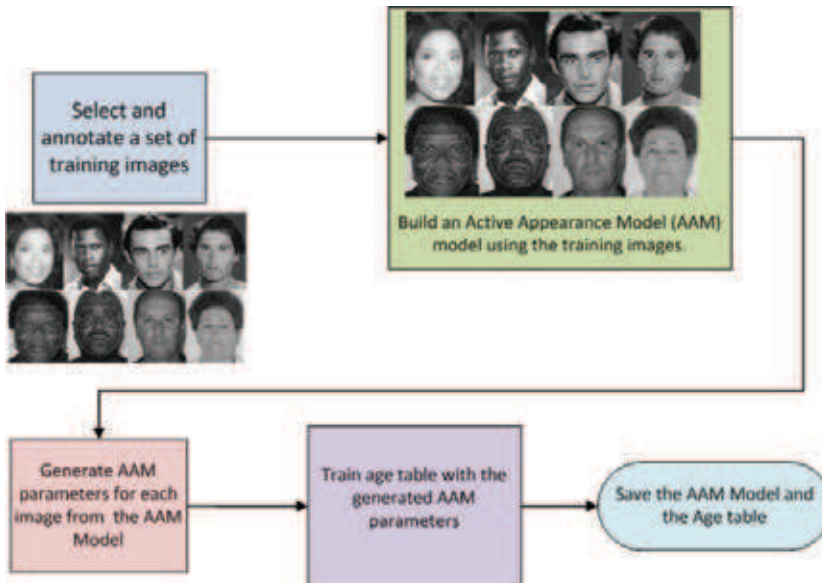
Fig. 6. Synthetic Facial Aging: Training phase
