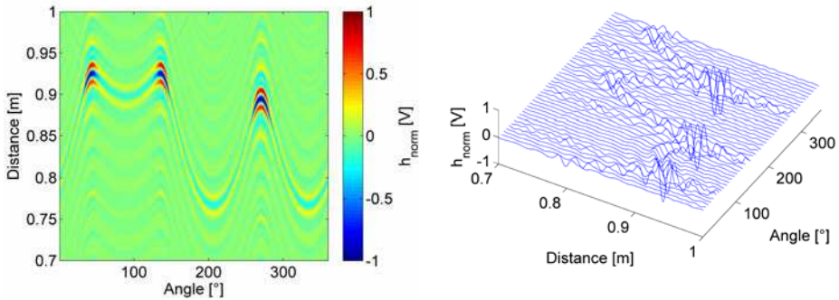
Fig. 4. Radargram of simulated object o3 (left) and every 8 th pulse of same Radar data (right)
