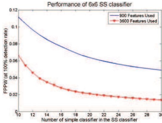
Fig. 6. Performance comparison of 6×6 classifier when using different feature sets
