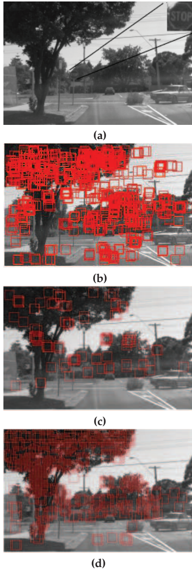
Fig. 5. Example output of SS and Half-DS classifier (a). Original Image. (b). Output of Half-DS classifier. There are a lot of false positives because there are 78320 windows to be processed per 376 \times 240 image. (c). Output of 3 \times 3 SS classifier. (d). Output of 6 \times 6 Classifiers
