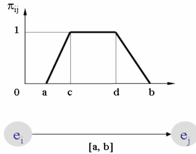
Fig. 1. Fuzzy temporal constraint set between two nodes e_i and e_j
