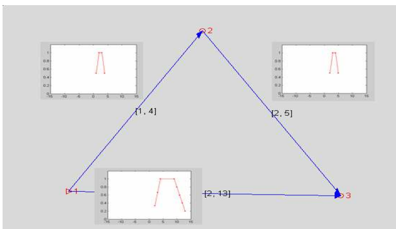
Fig. 5. Fuzzy temporal graph before minimization
