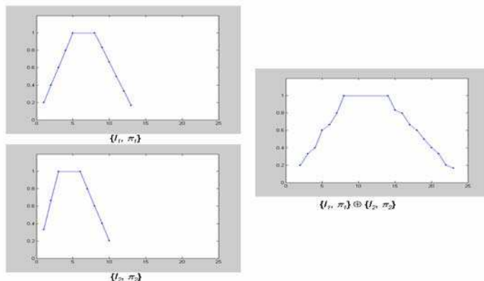
Fig. 4. Composition of two fuzzy temporal constraints
