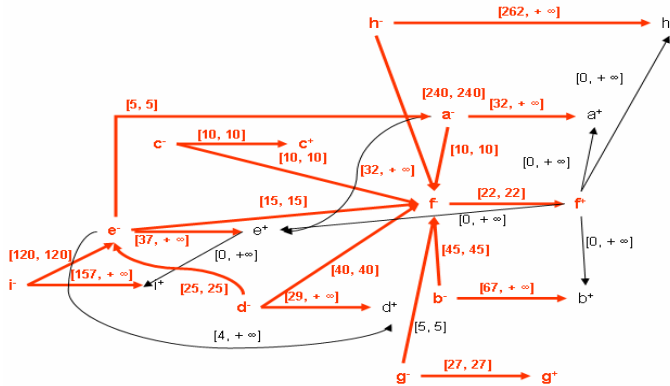
Fig. 21. Fuzzy temporal constraints of the coordinated plan at 12:22
