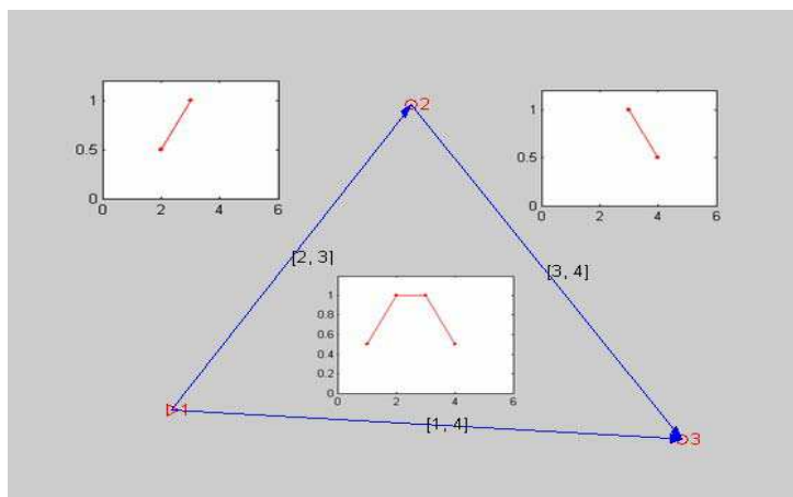
Fig. 7. Temporal inconsistency of a fuzzy temporal plan
