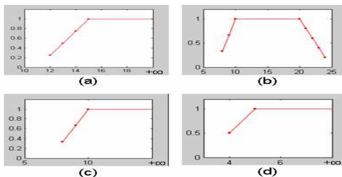
Fig. 14. Fuzzy temporal constraints in the sub-plans
