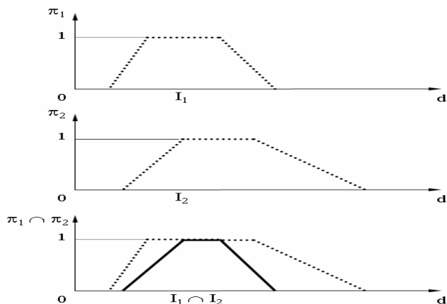
Fig. 3. Intersection of two fuzzy temporal constraints
