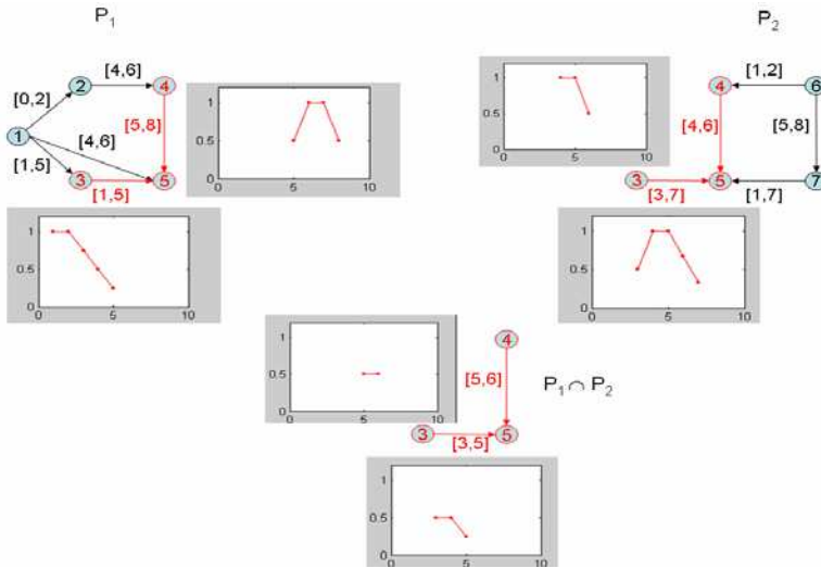
Fig. 8. Intersection of two fuzzy temporal plans
