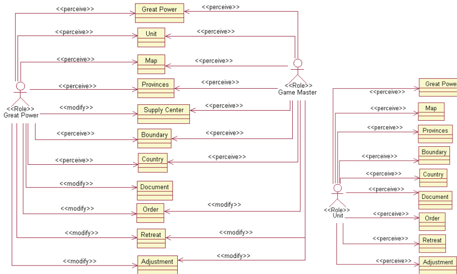
Fig. 9. Diplomacy game Environment Model
