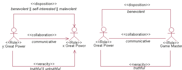
Fig. 6. Social behavior diagram showing relations between roles in the Diplomatic phase sub-organization (collaboration, veracity, and disposition)
