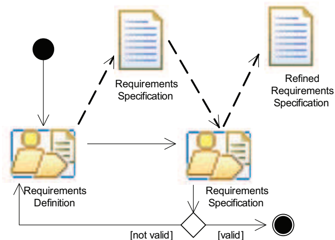
Fig. 2. Requirements modeling process overview
