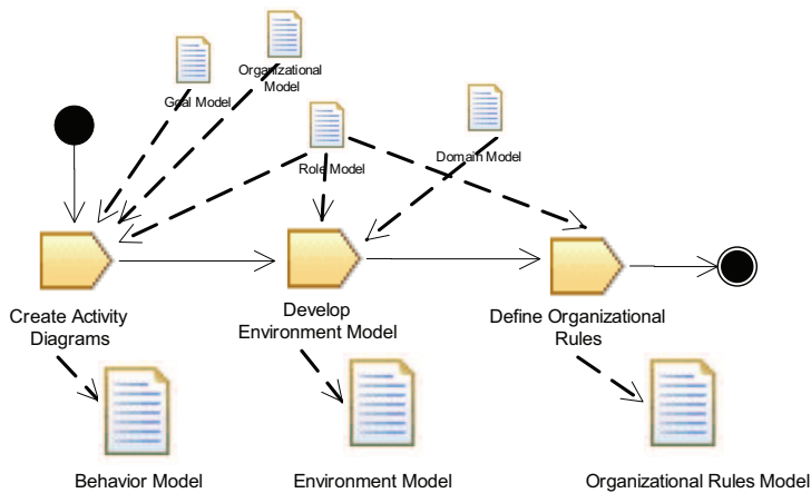
Fig. 4. Requirements Specification activity decomposed into tasks and artifacts
