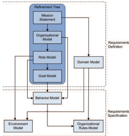
Fig. 1. Models of the proposal and its relationship
