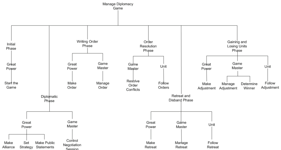
Fig. 5. Diplomacy game Refinement Tree
