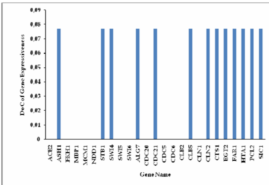
Fig. 12. Knowledge acquired by agents at t_6
