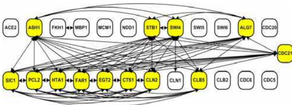
Fig. 14. Influence graph of KGS-based MCC behaviour at t_{17}
