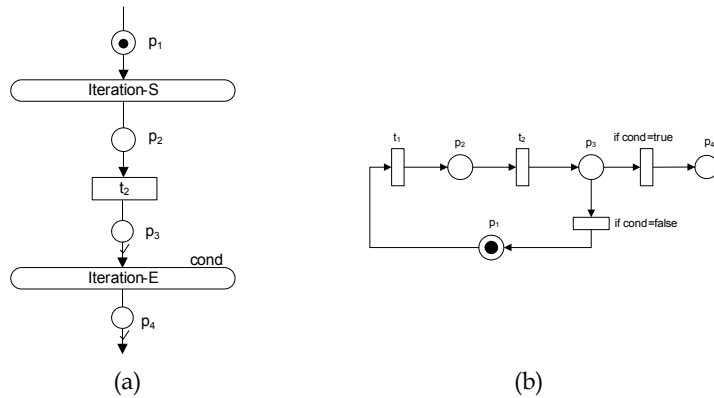
Fig. 8. Iteration (repeat...until loop)
