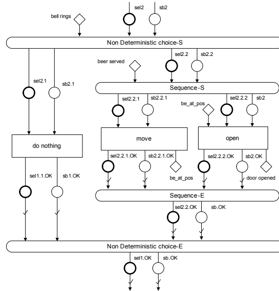
Fig. 14. Alternative actions according to Robbie's mental state
