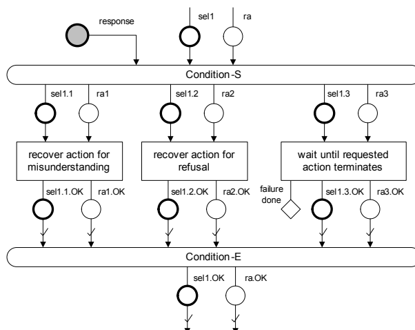
Fig. 12. FIPA-request protocol: send process
