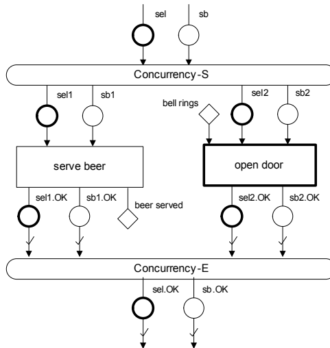
Fig. 13. Concurrent tasks for Robbie
