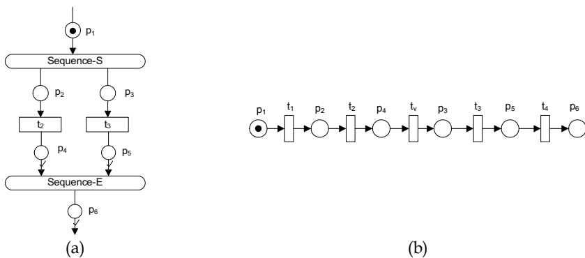
Fig. 4. Sequential execution
