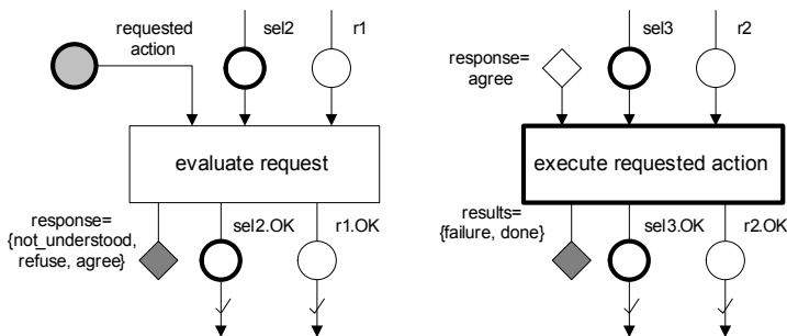
Fig. 11. FIPA-request protocol: receive process
