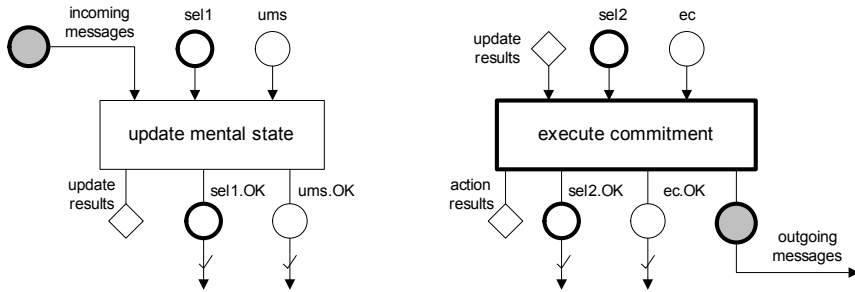
Fig. 10. Shoham’s generic agent interpreter
