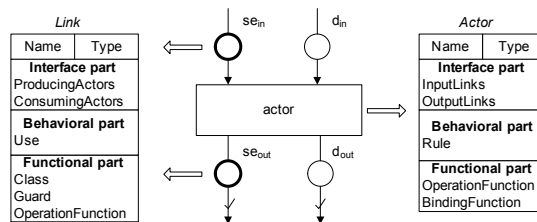
Fig. 3. The internal structure of actors and links
