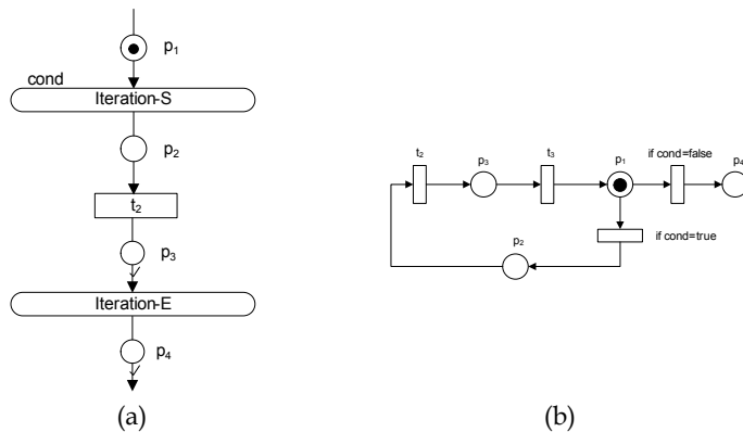
Fig. 9. Iteration (while...do loop)
