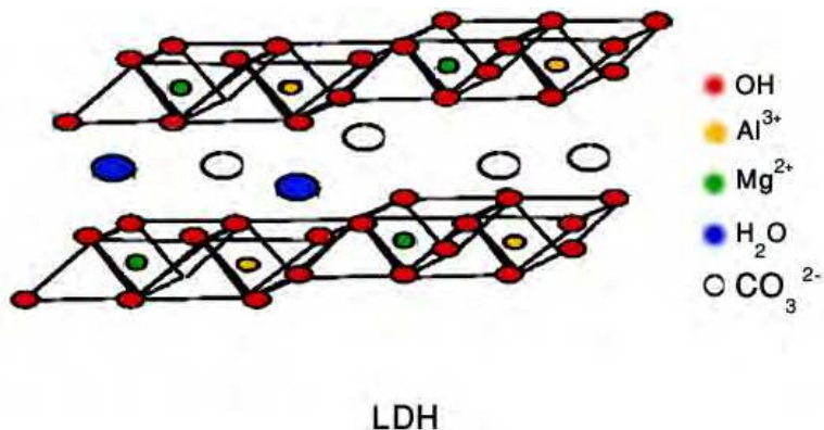
Fig. 14. Structure of layered double hydroxide
