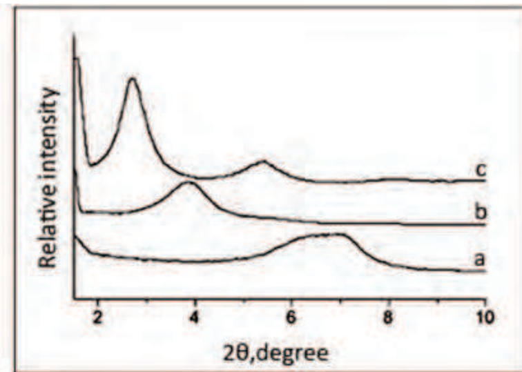
Fig. 4. XRD patterns of a) pristine sodium montmorillonite b) modified montmorillonite (OMT) c) ABS/OMT nanocomposite. ref:19
