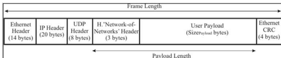
Fig. 6. Packet Format for the HIDL network within 'Network-of-Networks'
