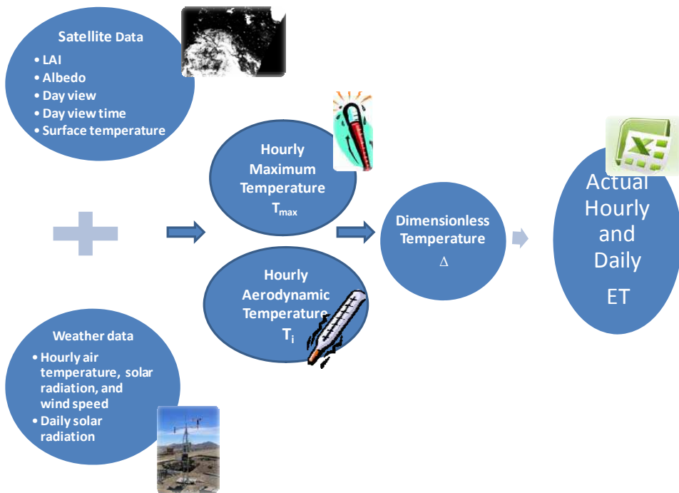
Fig. 1. ALARM and dimensionless temperature (ALARMMD) calculations of actual hourly and daily evapotranspiration.
