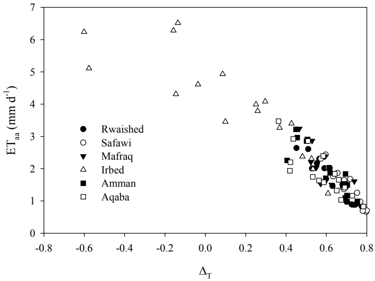
Fig. 9. Relationship between the ALARMD daily actual evapotranspiration ( ET_{aa} ) and the dimensionless temperature ( \Delta T ).
