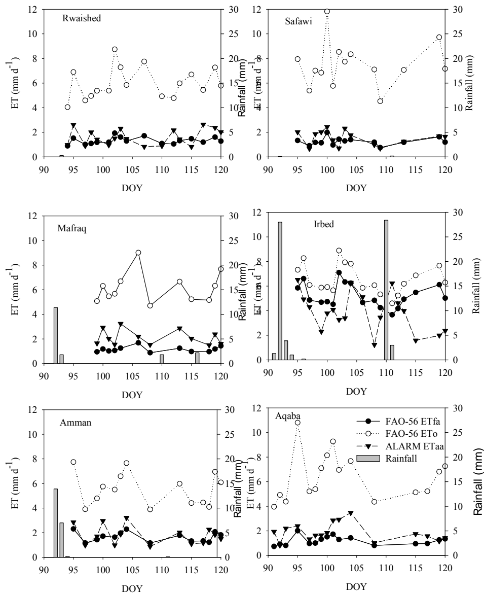
Fig. 8. Daily actual ALARM ( ET_{aa} ), FAO-56 ( ET_{fa} ) and FAO-56 grass reference ( ET_o ) evapotranspiration and daily rainfall amounts on different days of year (DOY) April 2005 for the six sites.
