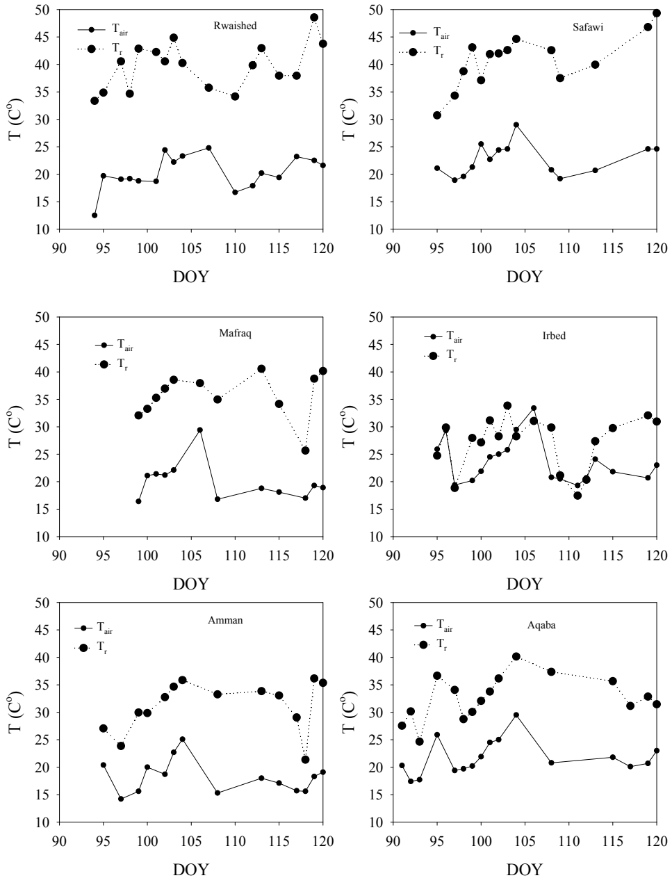
Fig. 6. Air ( T_{air} ) and radiometric surface temperature ( T_r ) on different days of year (DOY) during April 2005 for the six sites.
