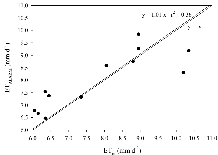
Fig. 4. ALARM vs. measured evapotranspiration at the validation site
