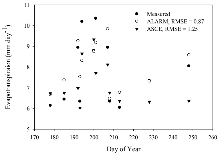
Fig. 3. Measured, ALARM and ASCE evapotranspiration at the validation site.
