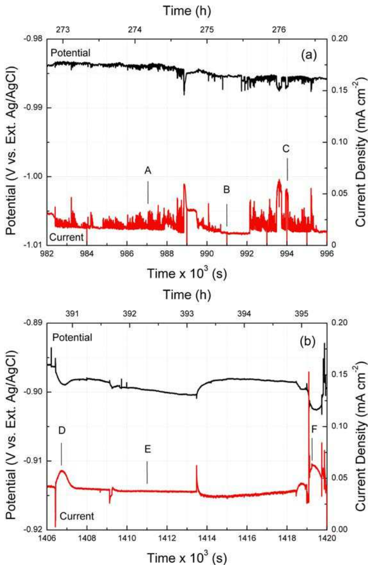
Fig. 5. Time records of the EPN and the ECN recorded in UCPN mode (a) for the lead caustic solution for the time period from 980 \times 10^3 to 996 \times 10^3 s, and (b) for that solution plus CuO for the time period from 1405 \times 10^3 to 1421 \times 10^3 s at 290 °C
