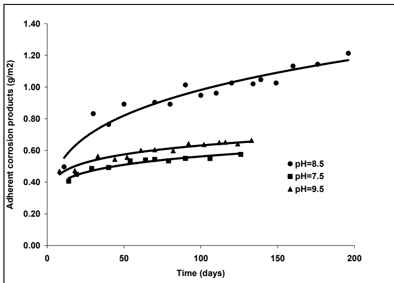
Fig. 8. Adherent corrosion products vs. time
