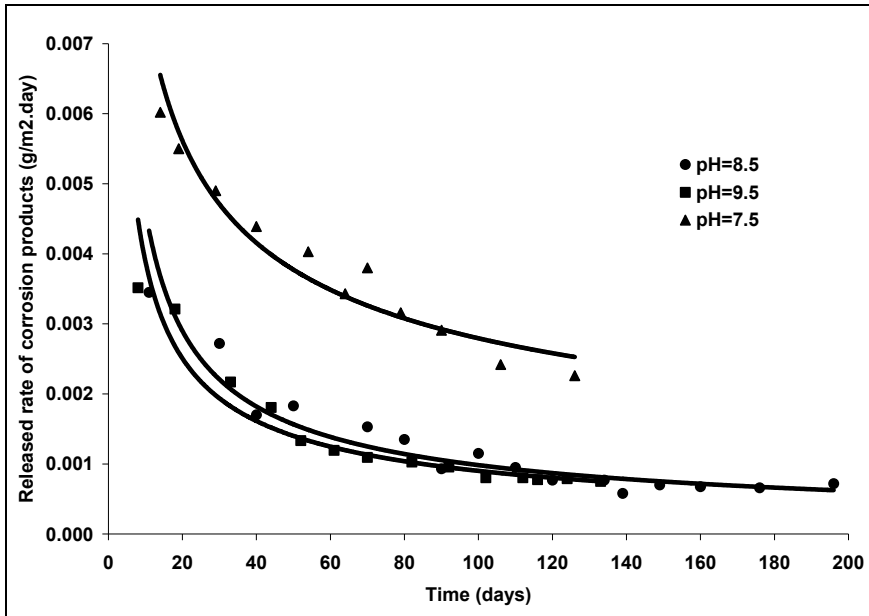
Fig. 10. Released rate of corrosion products vs. time
