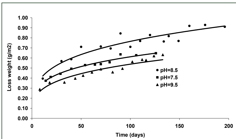
Fig. 5. Loss of metal by corrosion vs. time
