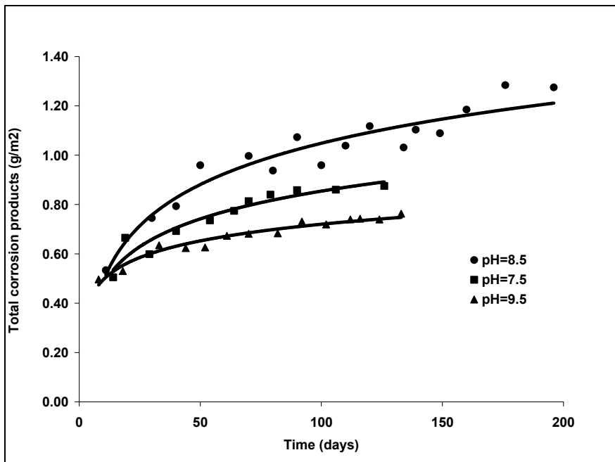
Fig. 7. Total corrosion products vs. time
