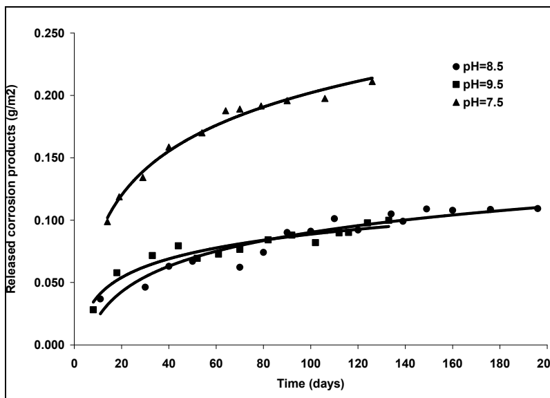
Fig. 9. Released corrosion products vs. time
