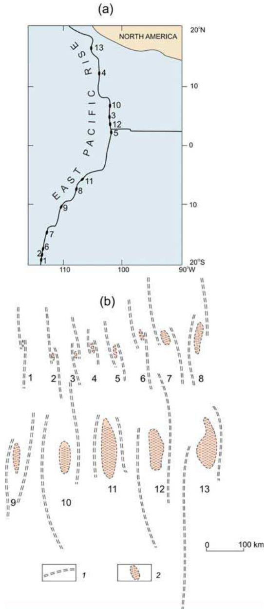
Fig. 3. Geometric self-similarity of overlapping spreading centres (OSC) at the ridge of the East Pacific Rise: (a) OSC locations; (b) their generalized morphotectonic schemes, based on comprehensive investigation of the submarine topography. (1) axes of spreading centers, (2) structural depressions between them, after [29].
