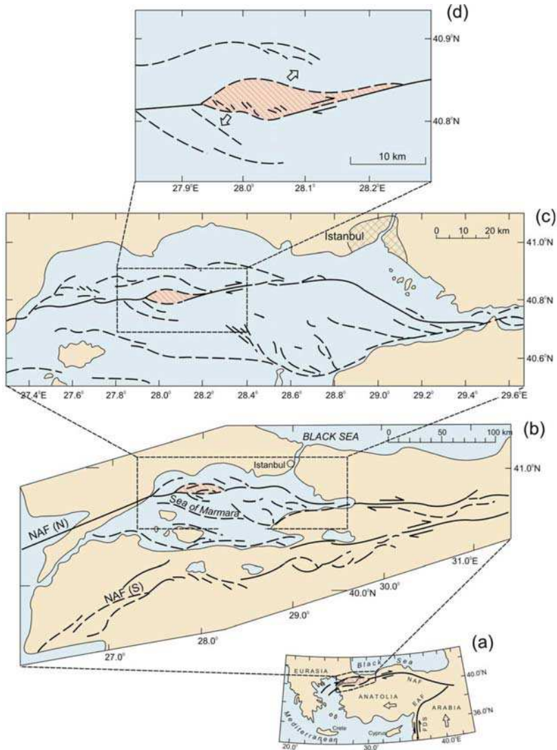
Fig. 1. Fractal structuring by the example of scale-invariant pull-apart structures of the Sea of Marmara and its framing after [16]. (a-d) sequential scale extension: (a) splitting of the North Anatolian Fault - NAF(N) and NAF (S) dividing the Anatolia Microplate from the Eurasian Plate. (FDS) Fault of the Dead Sea, Arrows show moving directions of plates and displacements along faults. (b) pull-apart basin of Sea of Marmara and different in rank rhomb-like or oval pull-apart structures along (N) northern and (S) southern branches of the North Anatolian Fault. Solid and dotted lines indicate main and general faults accordingly; and arrows, displacements along faults. (c) pull-apart structures of the northern branch; (d) one of rhomb-like local young depressions; arrows show displacements along the fault and the direction of the depression's opening.
