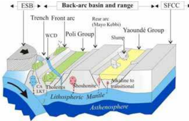
a) Pre-orogenic setting: subduction / back-arc basin and range setting (1000-640 Ma)
