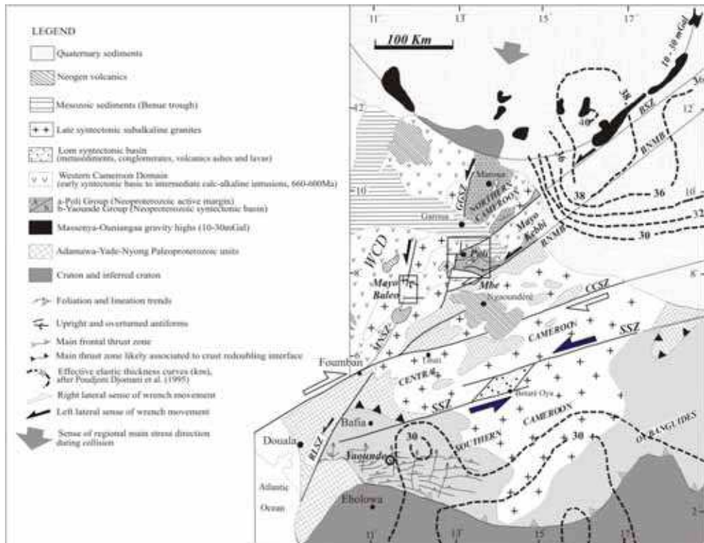
Fig. 2. Structural map of the Cameroon domain (see location in Fig.1)
