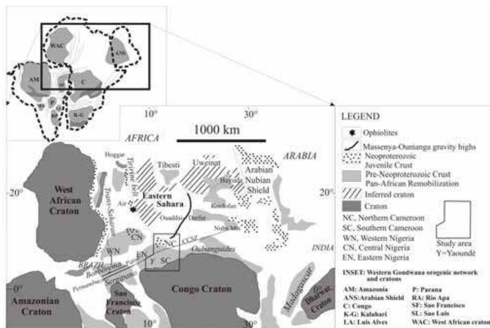
Fig. 1. Sketchy tectonic map of western Gondwana and main geotectonic units (redrawn from Küster & Ligeois, 2001)
