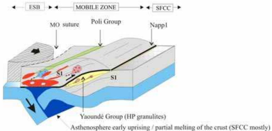
b) PHASE D1: crustal redoubling and thickening-early thrusting/nappe1 ( 640-630 Ma)
