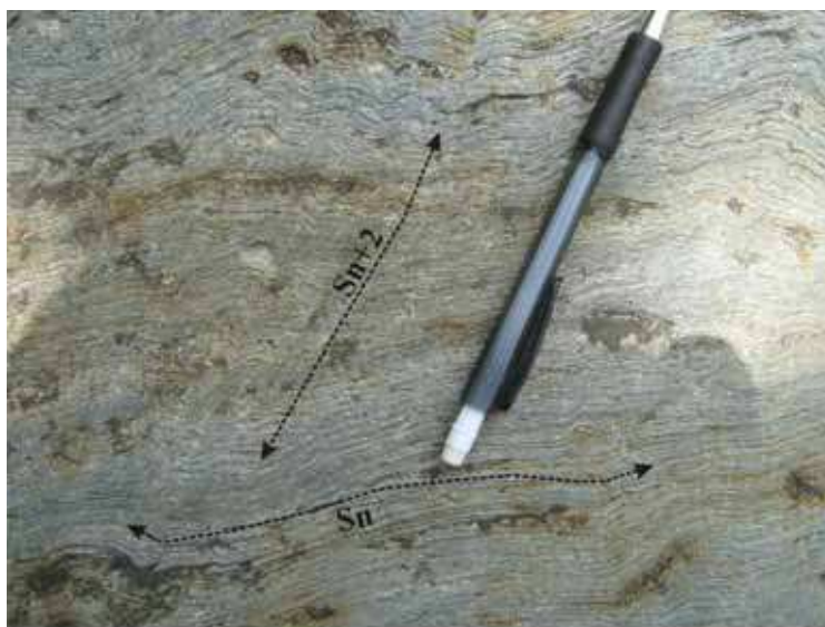
Fig. 6. Crenulation cleavage associated to Late Pan-African folding ( F_{n+2} or F_3 ) in northern Cameroon (Poli Group)
