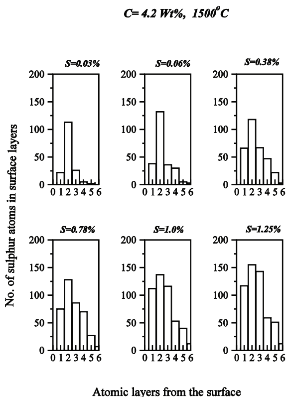
Fig. 11. Concentration of sulphur in the top five surface layers in a liquid bath configuration (24x24x15). Results for C = 4.2 wt%, T = 1500^\circ \text{C} have been presented. Corresponding bulk sulphur values ranging from 0.03% to 1.25% have also been shown above individual bar plots.
