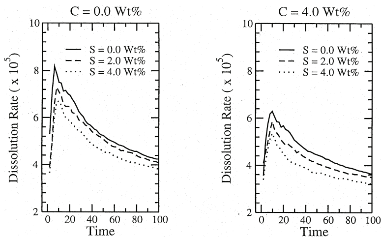
Fig. 5. Carbon dissolution rate as a function of time, across basal plane for a range of carbon and sulphur concentrations in the melt.
