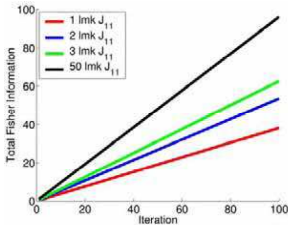
Figure 3. First entry in the total Fisher information matrix ( \sum \sum \zeta_{ij} ) for a monobot with variance parameters P_{r,0|0} = \mathbf{Q} = \mathbf{R} = 1 , and various sizes for the measurement vector
