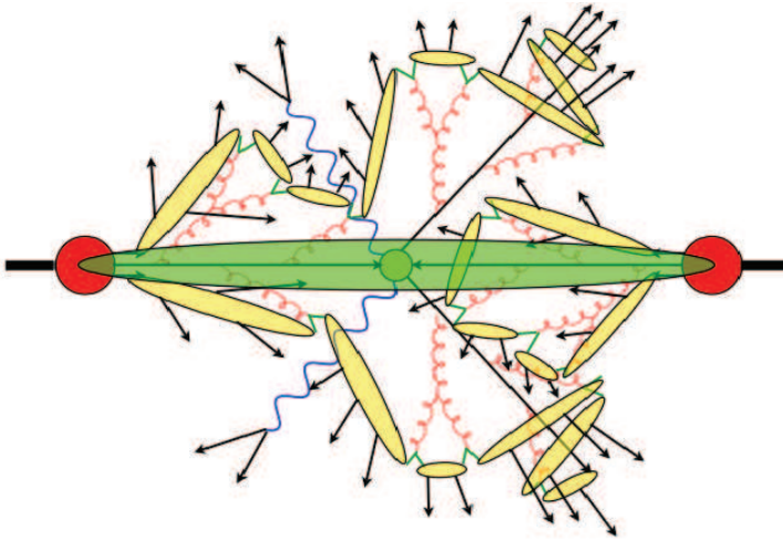
Fig. 1. LHC Monte Carlo evolution described by HERWIG program. Two protons are incoming. A proton is made of three quarks. A generation of Standard model particles is produced. Quarks are yellow and gluons are red
